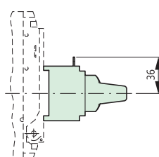
NZM1-XDTV
