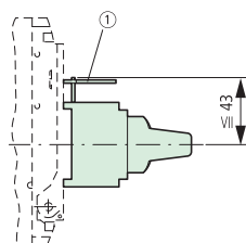
NZM1-XDV NZM1-XDVR
