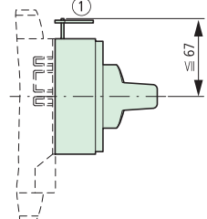
NZM2-XDV NZM2-XDVR
